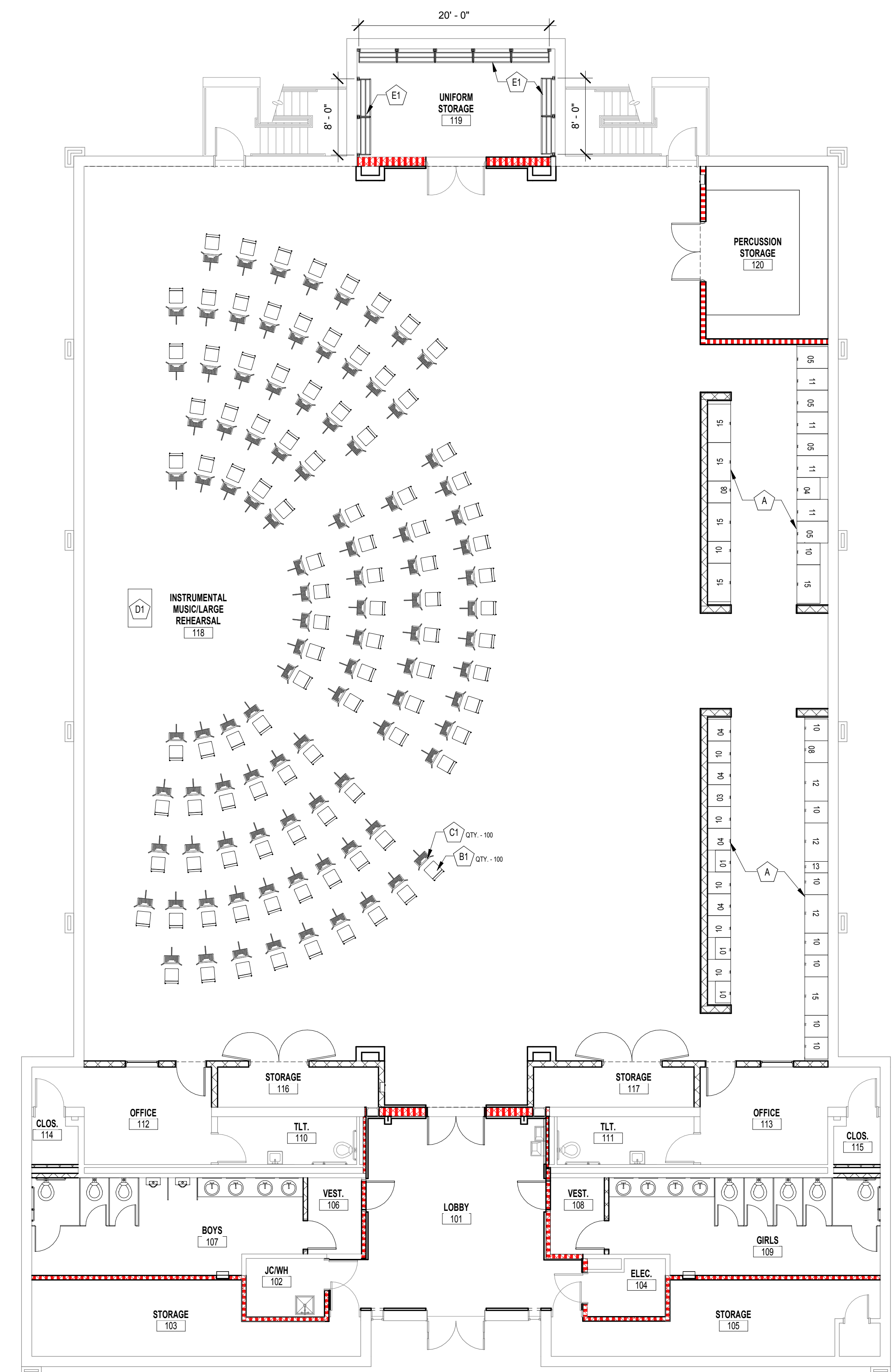
1 FURNITURE PLAN 1/8" = 1'-0"
